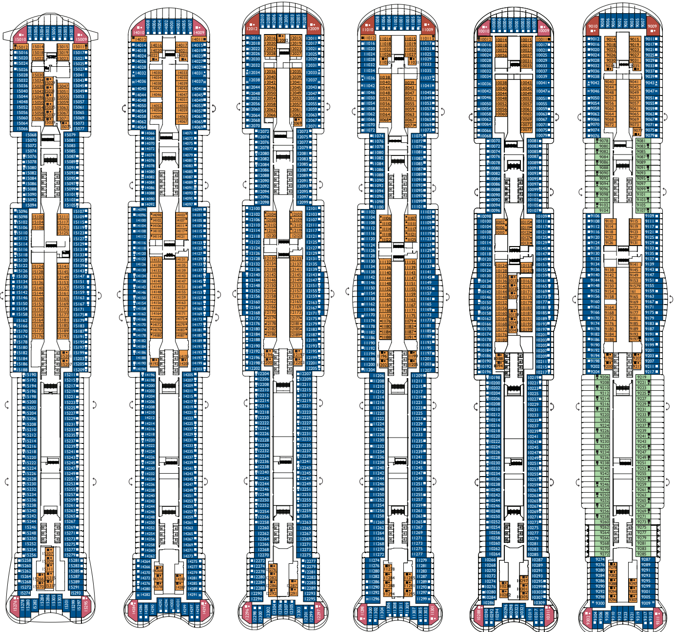
DECK 15 MILANO
